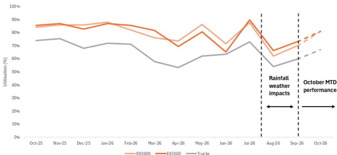
Figure 2: LTM excavator and truck fleet utilisation demonstrating the impact of rain events on utilisation in August & September
