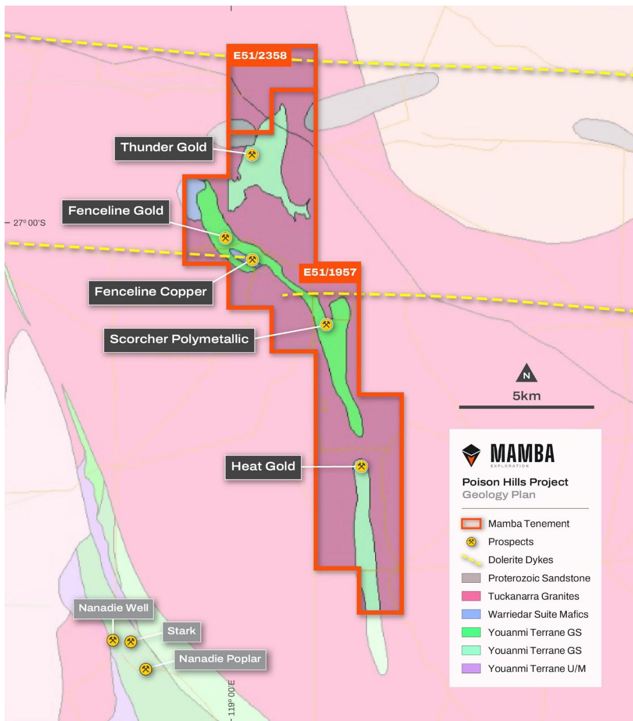
Figure 2: Poison Hills Geology Map with Prospects
