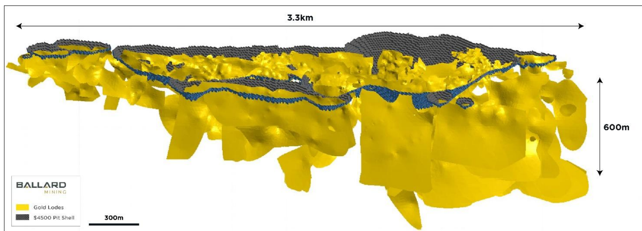
Figure 4 – Three-dimensional view of the 1.36 Moz Baldock deposit looking NE showing the open pit shell (A$4,500/oz) containing 516 koz of gold and Mineral Resources reported below the open-pit shell within interpreted lodes and constrained within optimised underground reporting shape containing 847 koz
