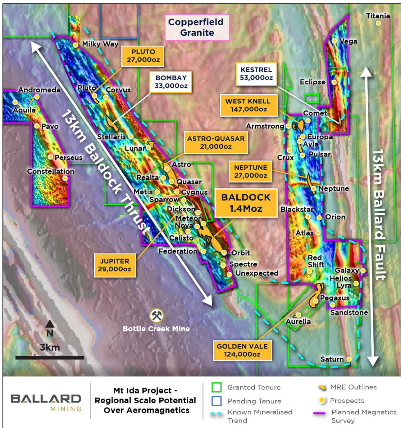
Figure 9 - Aeromagnetic image showing the existing 53 exploration targets within Ballard Mining's tenure
