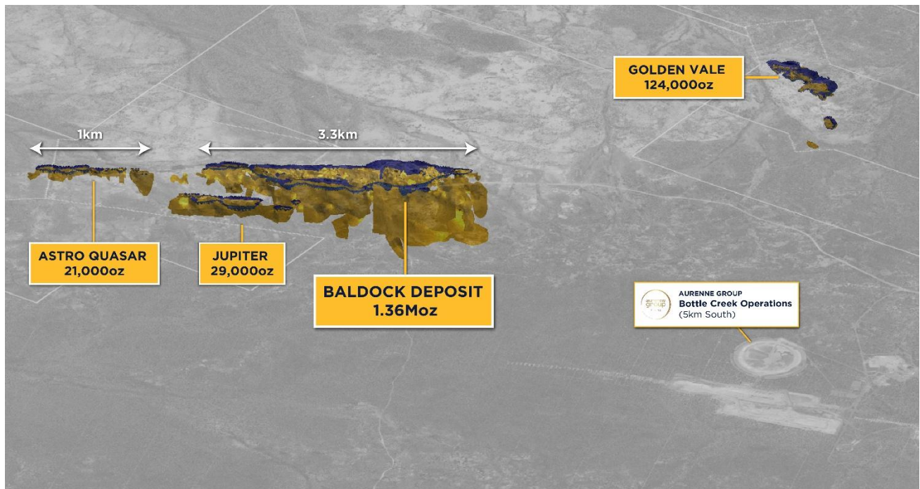
Figure 3 – Aerial view of Mt Ida gold project looking northeast across semi-transparent surface imagery showing the 1.36 Moz Baldock, 124 koz Golden Vale, 29 koz Jupiter, and 21 koz Astro-Quasar gold deposits with the Aurenne Group's Bottle Creek Operations in the foreground.
