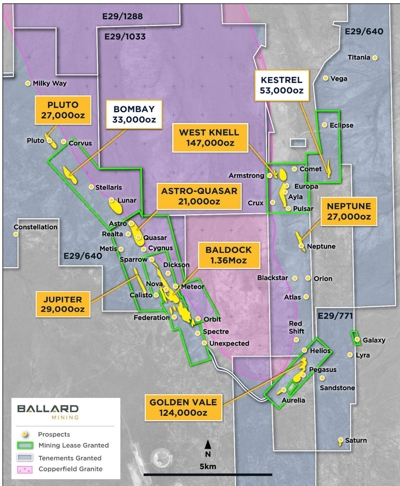
Figure 2 – Mt Ida Project Plan showing deposit locations and updated Mineral Resource Estimates (oz).
