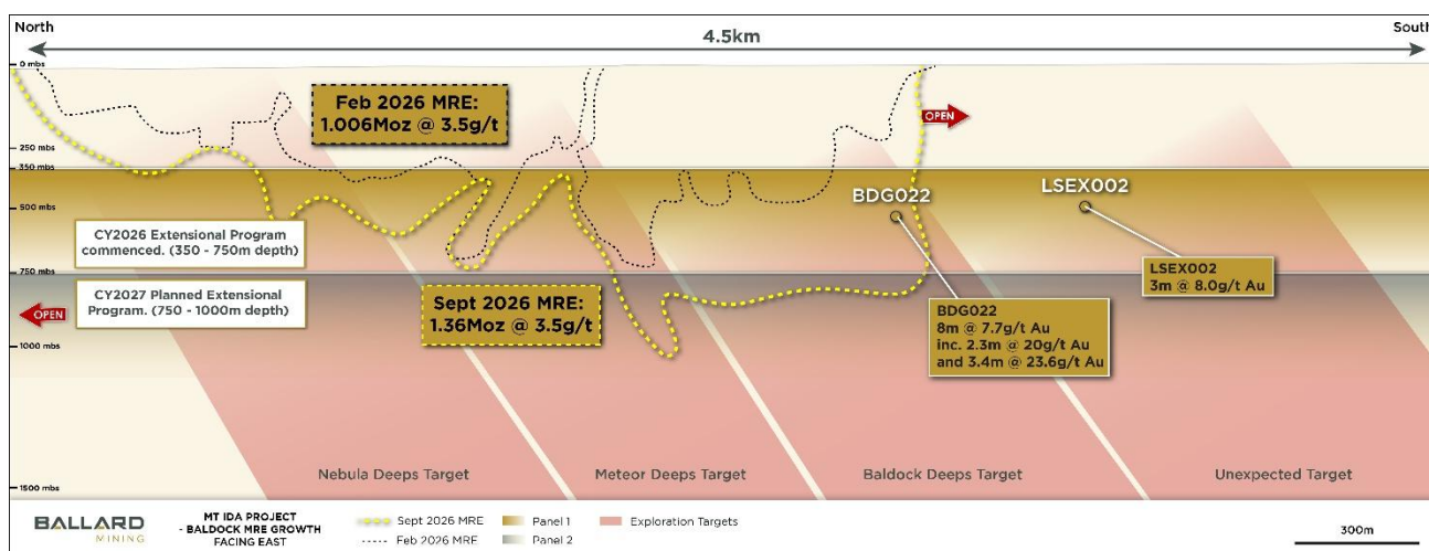
Figure 5 - Long section of the Baldock Mineral Resource outline change from February 2026 to September 2026
