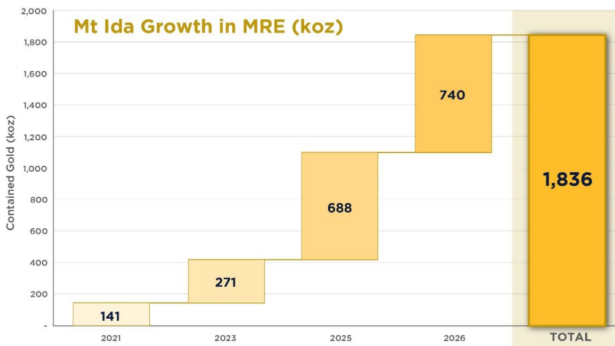
Figure 1 - Waterfall chart showing the increases in the Mt Ida gold resource since acquisition by Red Dirt Limited in Sep 2021, subsequently renamed Delta Lithium Limited in 2023, and demerging the project into Ballard Mining Limited in 2025.
