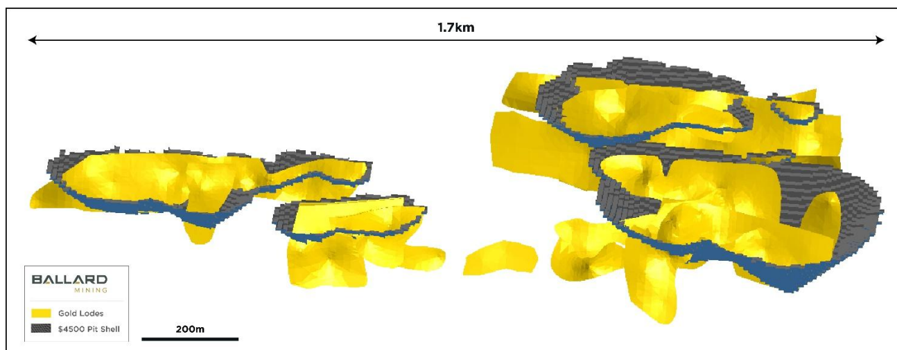
Figure 6 - Isometric view of the West Knell deposits showing open pit shells (A$4,500/oz) and containing 147 koz of gold and extensive gold mineralisation down to 250m vertical depth. Mineralisation is open along strike and at depth.
