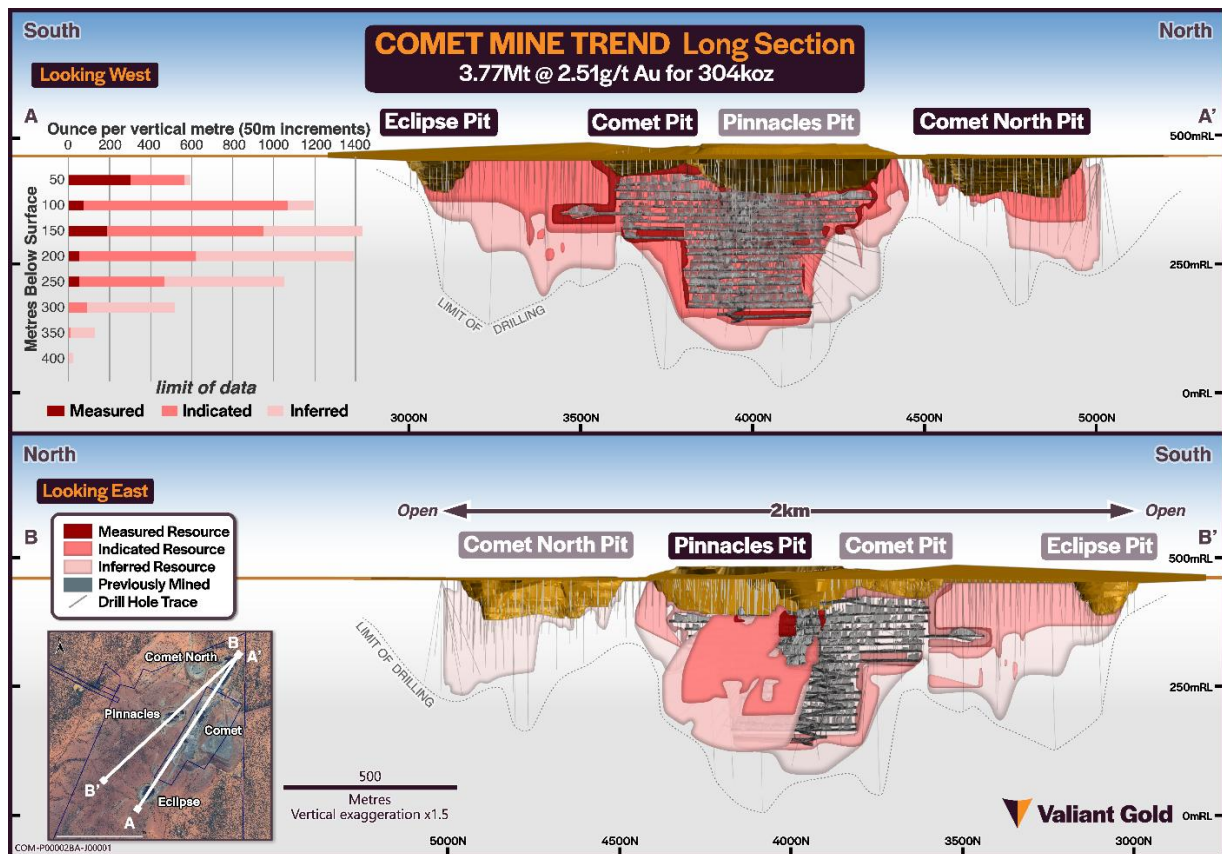
Comet Mine Trend schematic long section, facing west, showing the Mineral Resource Estimate, ounce-per-vertical-metre distribution and previously mined volumes. 1
