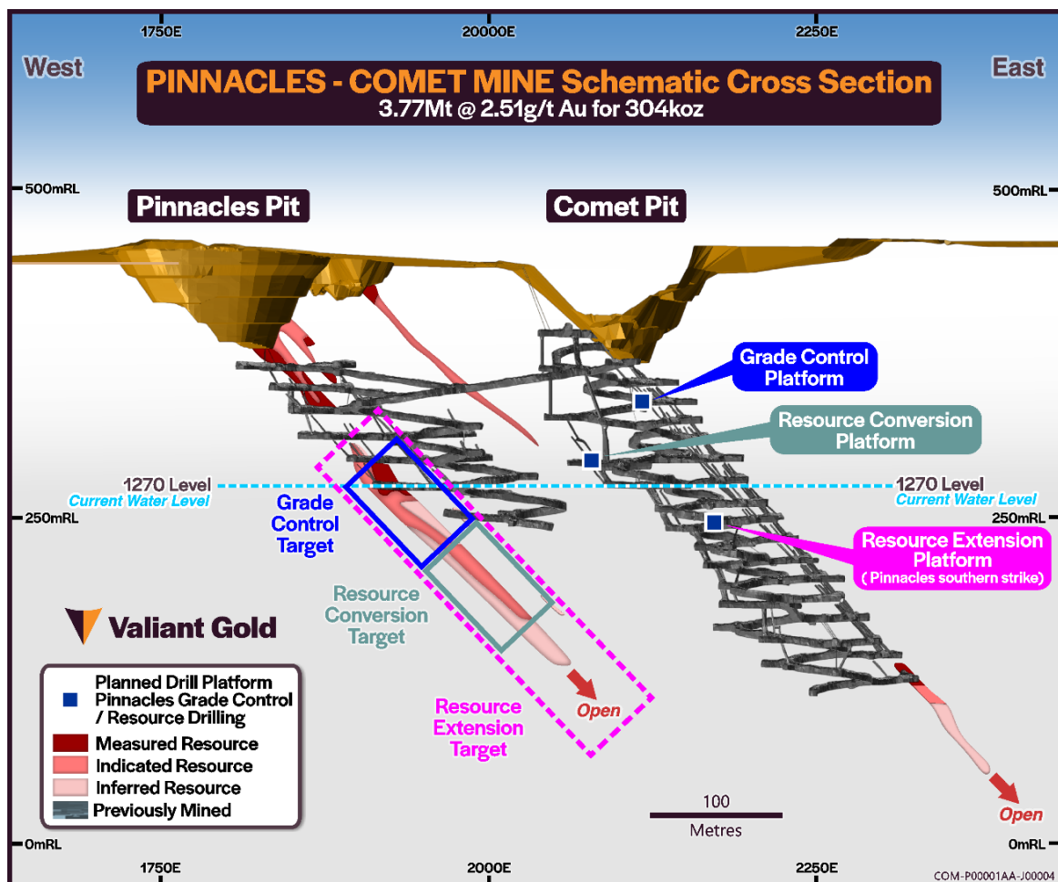
Figure 2: Comet Mine schematic cross-section showing the underground mine workings, Mineral Resource Estimate outline and classifications, planned drill platforms, and priority grade control, resource conversion and resource extension drilling areas. 1
