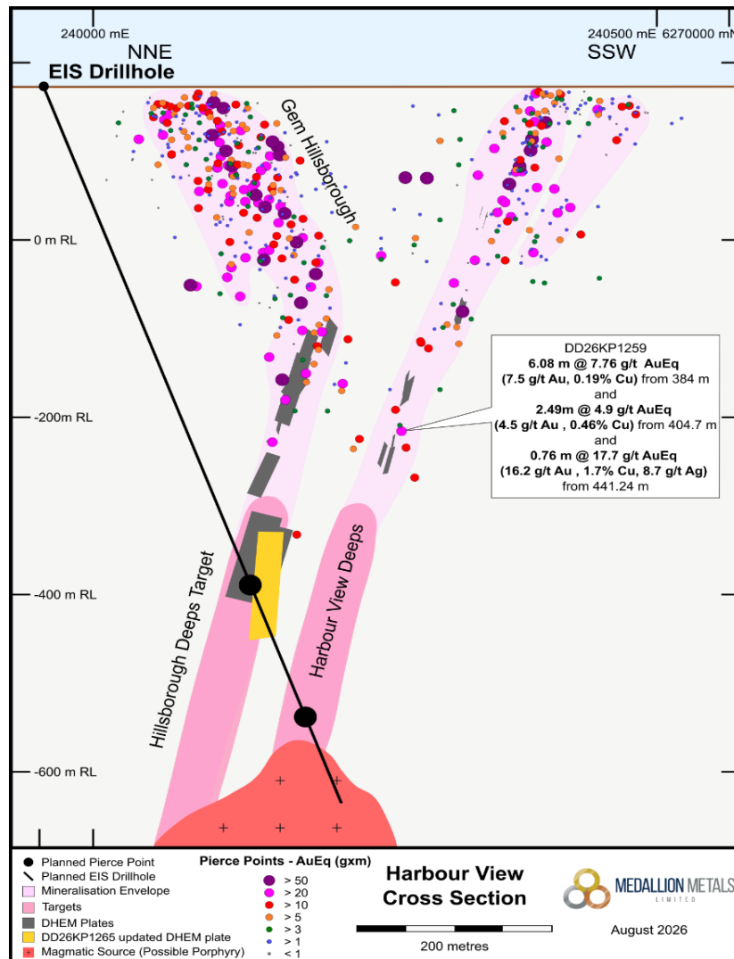
Figure 1: Hillsborough Deeps/Harbour View cross section showing reported drilling results and mineralised trends. 7
