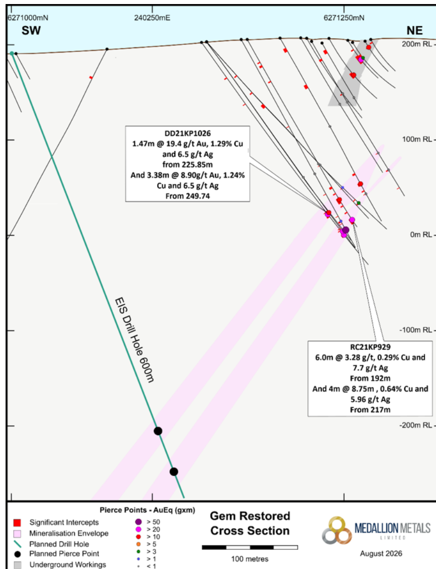
Figure 2: Gem Restored cross section showing historical drilling results RC21KP929 8 and DD21KP1026 9 and planned EIS drill hole.
