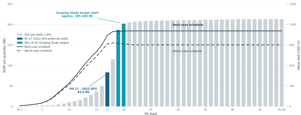
Figure 4: Pit optimisation results: pit shell tonnage and schedule value add, with the 2022 DFS preferred shell (Pit 17) and the Scoping Study target shell (Pits 19 to 20) highlighted. Source: adapted from Steelpoortdrift Project DFS, Figure 0-7 (Sound Mining International, 2022); values digitised from the 2022 DFS figure, indicative.
