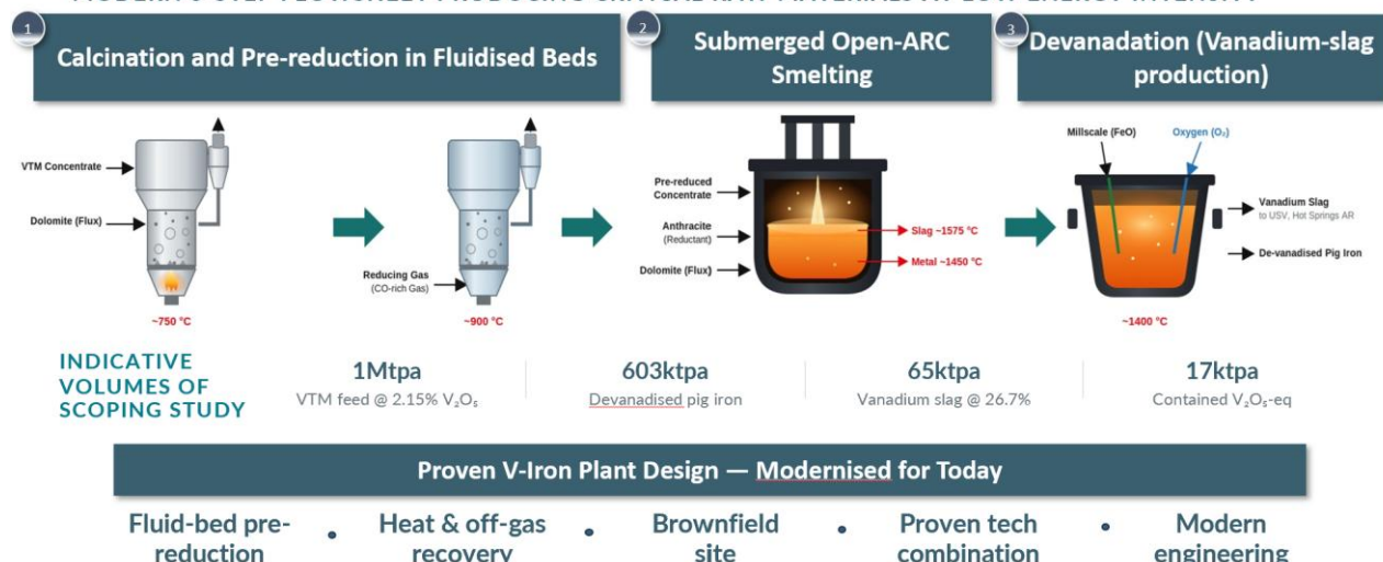
Figure 2: Basic Flowsheet of the proposed V-Iron processing route.
