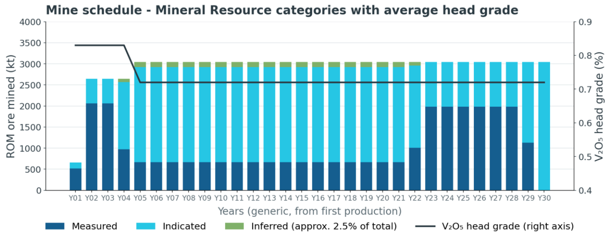
Figure 5: Mine schedule by Mineral Resource category with average head grade, 2022 DFS mine plan applied on the accelerated V-Iron schedule; category make-up re-phased from the 2022 DFS mine schedule (Sound Mining, 2022) by cumulative tonnage, indicative pending the V-Iron DFS mine schedule.
